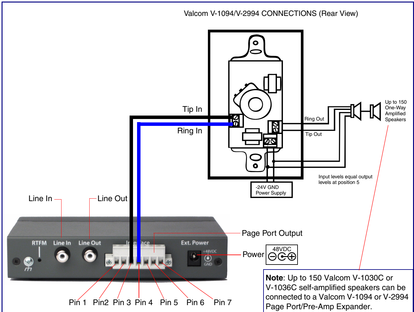
Figure 1. SIP Paging Adapter to Valcom V-1094/V-2994 Connections
